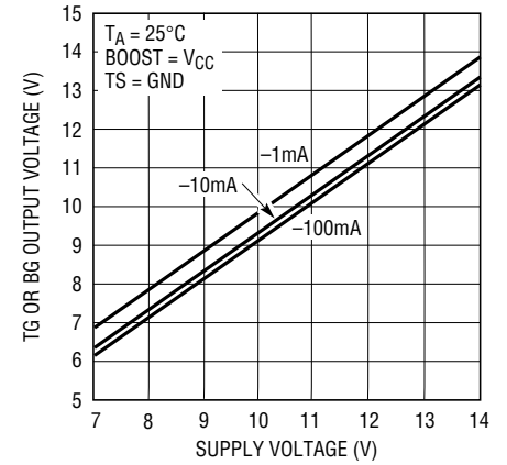
Output High Voltage (VOH) vs Supply Voltage
